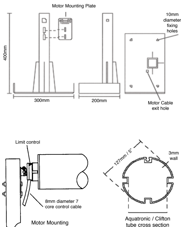
Aquatronic Roller - Dual Purpose Bracket Motor & Non Motor End Support
