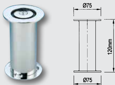
Level Anchor Fixing - Dia 43mm
