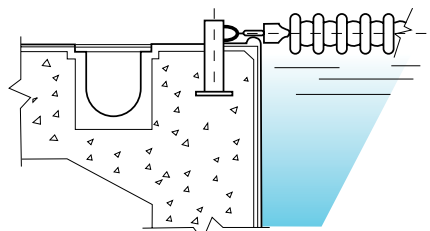
Level Anchor Installation CEMLA43 - Level Anchor CEMFLS - Float Line Support
