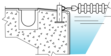
Inclined Anchor Installation (5° Angle) CEMLA43 - Level Anchor CEMFLS - Float Line Support
