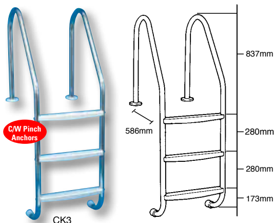
Certikin 1.5" / 38mm Ladders For Concrete Pools
