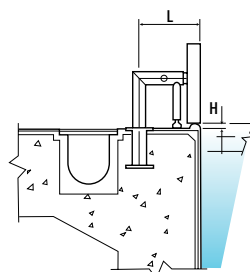
Installation Type A Position of fixings when dimension 'L' is over 500mm
