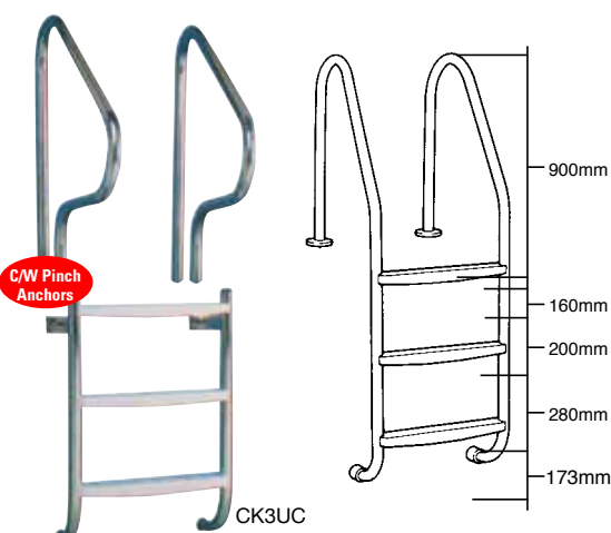
Certikin 1.5" / 38mm Undercover Ladders - C/W Grabrails (Pinch Anchor fixing included)
