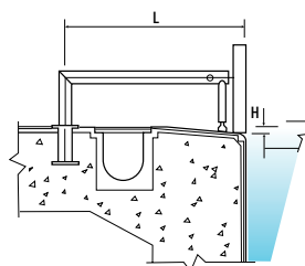
Installation Type A Position of fixings when dimension 'L' is over 500mm
