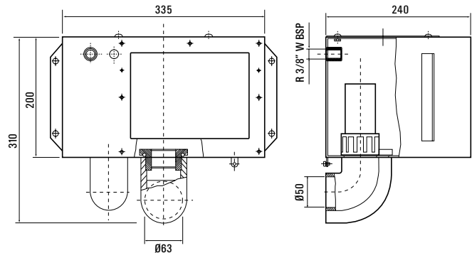
Stainless steel skimmer - CKSS520
