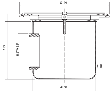
Stainless Deck Box CKSS393
