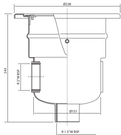
Stainless Main Drain CKSS196
