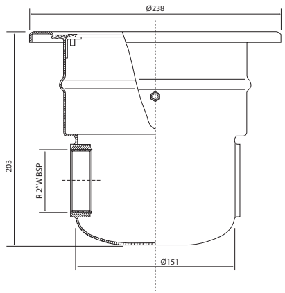
Stainless Main Drain CKSS268
